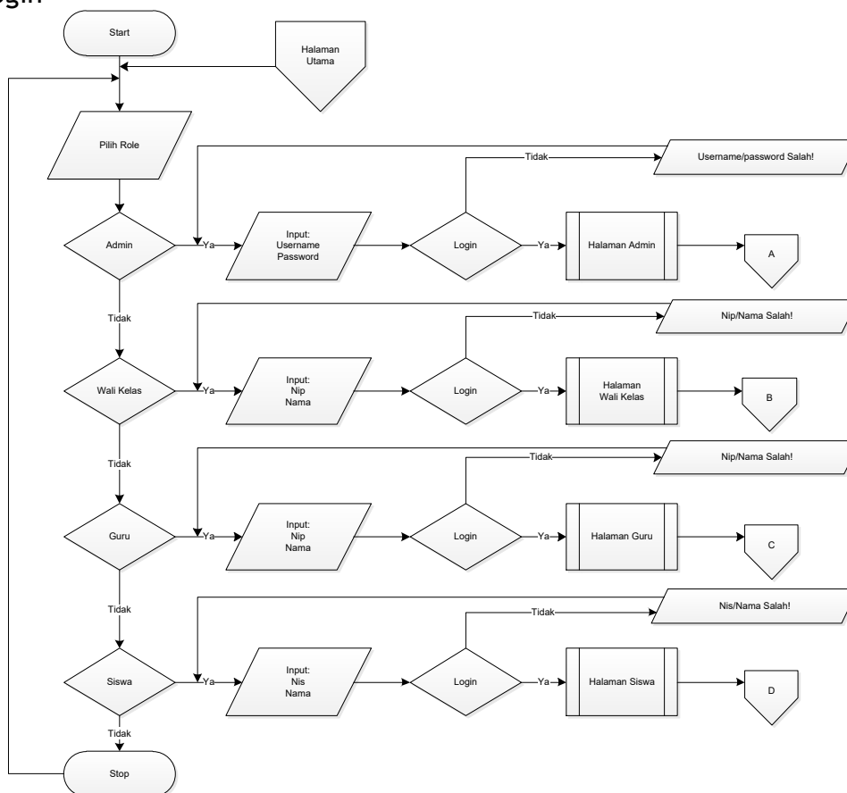
Gambar 1. Flowchart login
