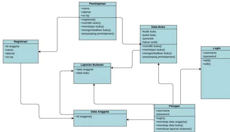
Gambar 3.8 Class Diagram
