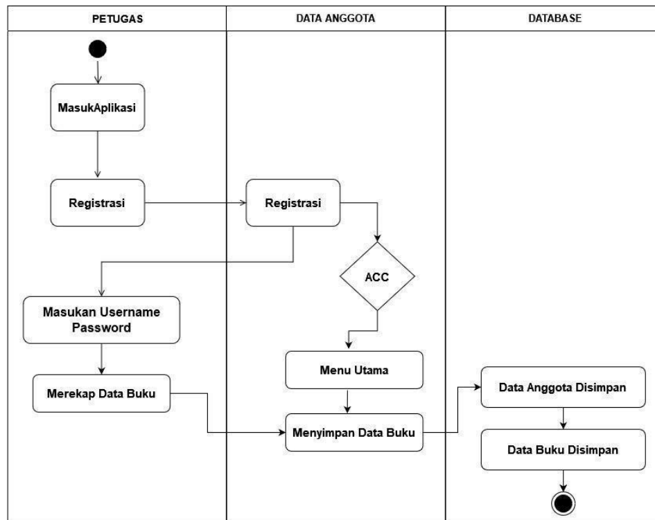
Gambar 3.10 Activity Diagram
